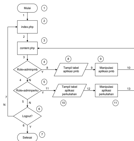
Fig. 3.3 Flowchart Program Administrator
