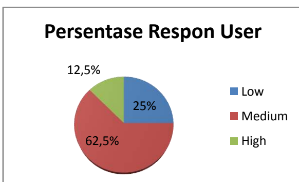
Fig.9 Graph of Percentage of Observations
