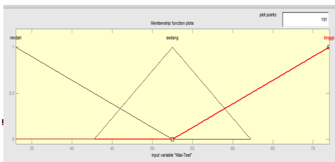
Image 4.4 The curve of the function value of high membership Variable degrees of written Test
