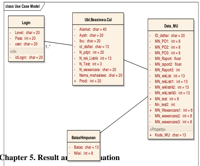
Image 3.10 Class Diagram of Scholarship SPK
