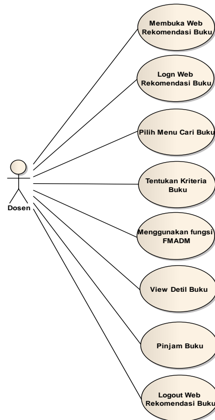
Fig 7. Search book
